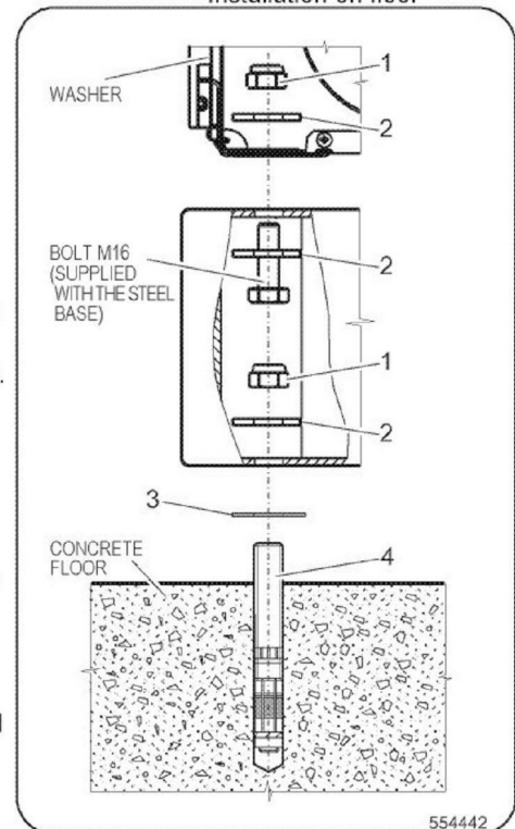
Figure 15 – Rigid-mount machines, Installation on a steel base and floor
