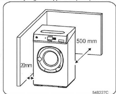
Figure 9 – Rigid-mount machines
