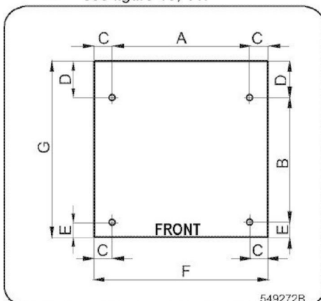
Figure 10 – Rigid-mount machines
