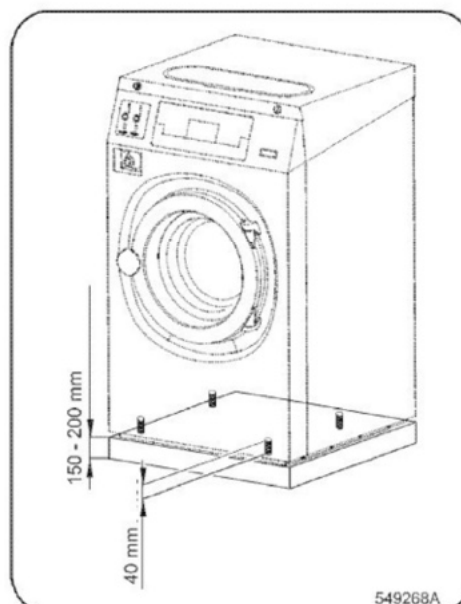
Figure 12 – Rigid-mount machines
