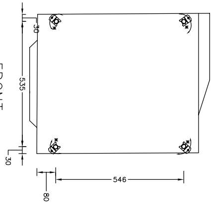
FOOTPRINT
