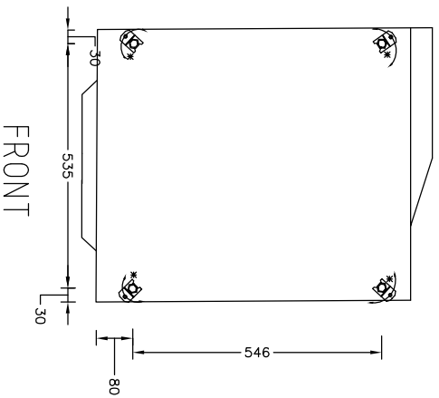
FOOTPRINT
