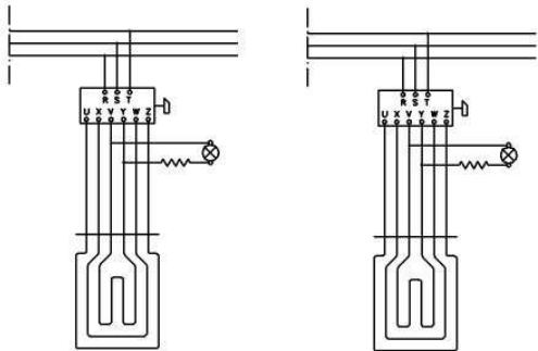
PLATE 300x300mm Kw 2,4
