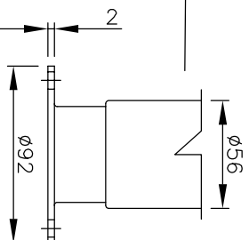
FOOT DETAIL
